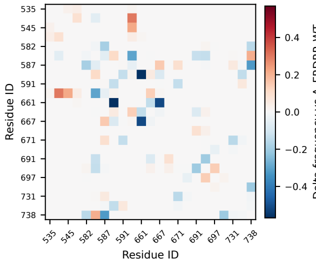
C: BMS-986205 / WT (Success)
